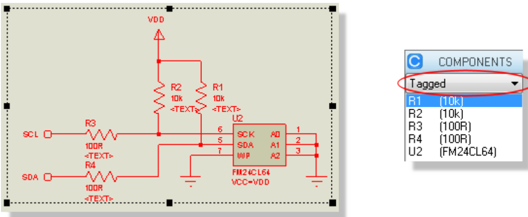
Components selected on the schematic can form a filtered placement list on the layout.
