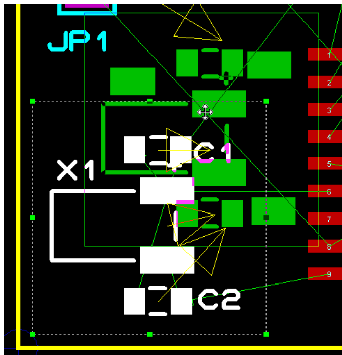
Moving a selection of circuitry
