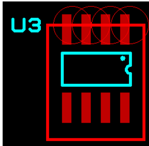
U3 with a Keepout
