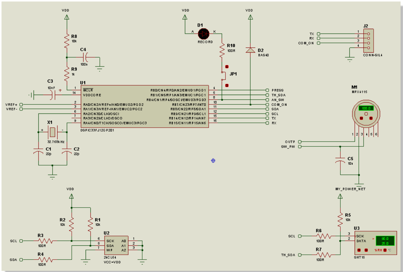
Completed dsPIC33 circuit
