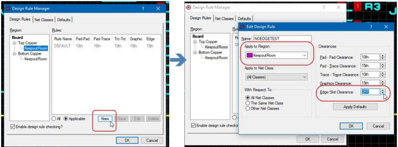
Setting a new Rule for the Design Room.
