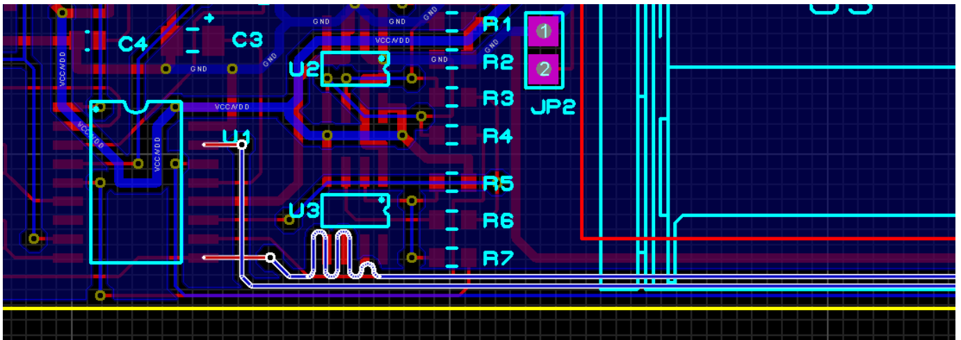
Matched lengths
