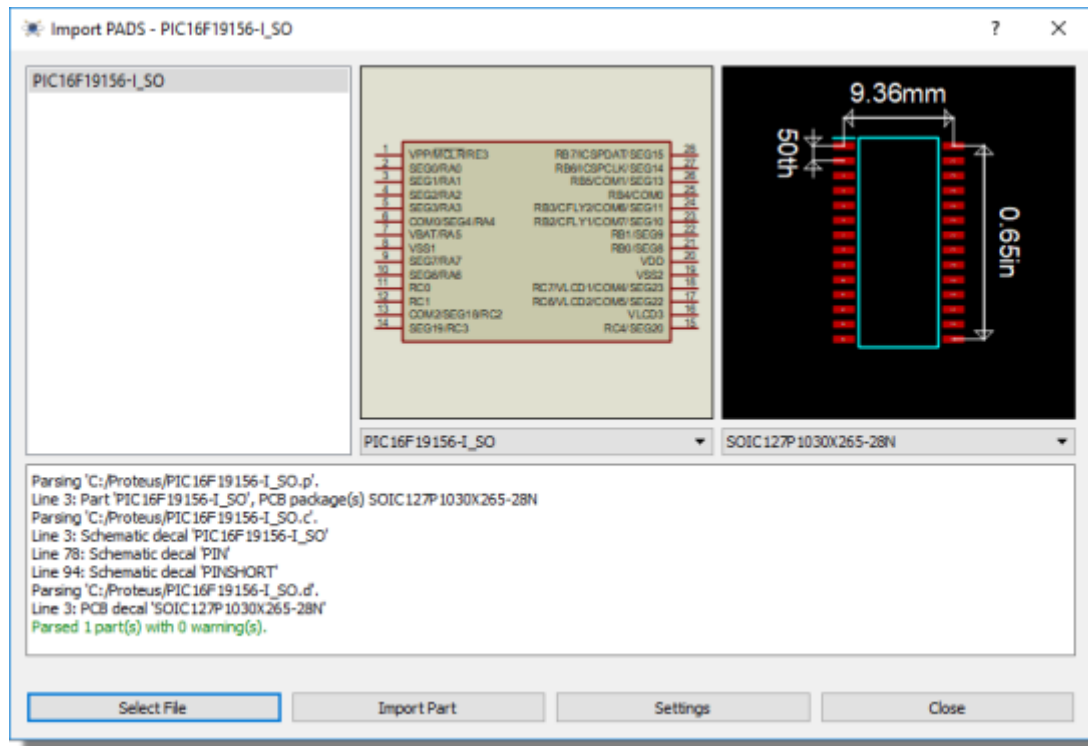
The Import Part dialogue with a part loaded.
