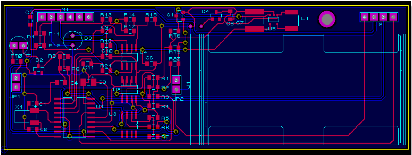
Power Plane has flooded the entire layer
