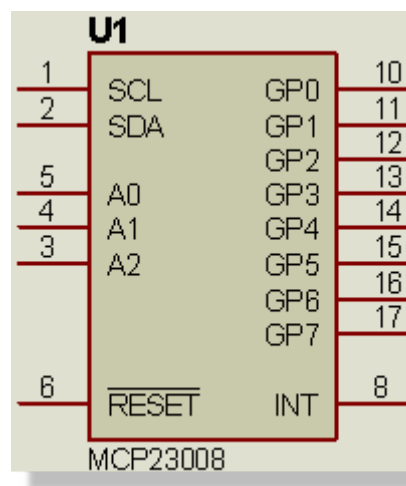
The MCP23008 Completed
