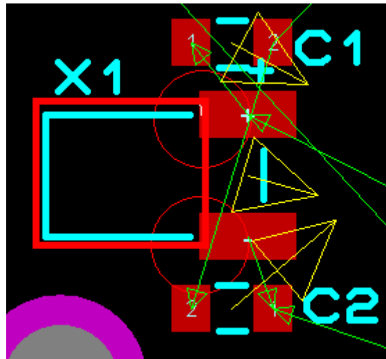
Keepout placed produces 2 DRC errors
