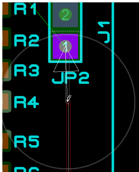
Connecting to JP2 Pin 1
