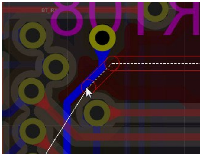
Visual DRC Auras around Tracks and Vias when placing a route.
