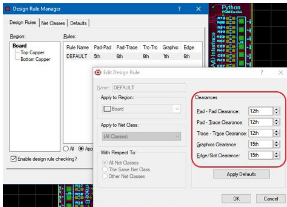
Default clearance settings in the DRC manager
