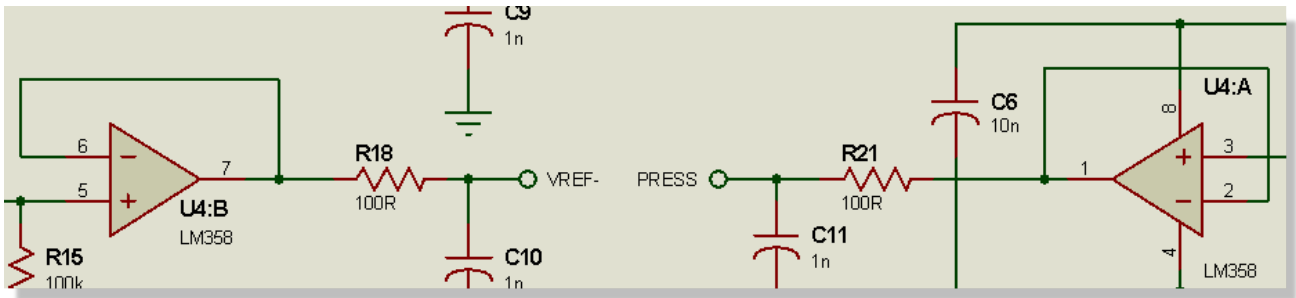
U4:A and U4:B
