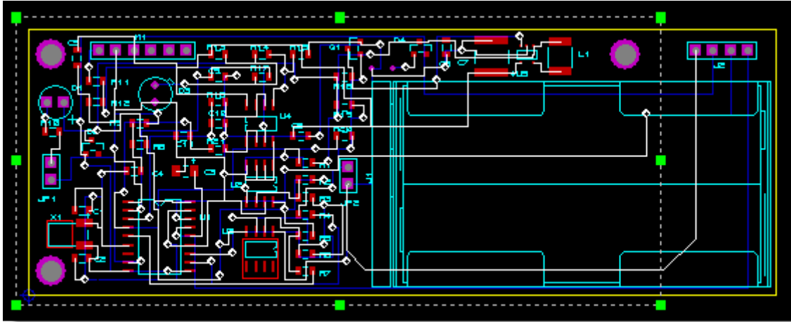
Notice that Only the traces on Top Copper are Selected
