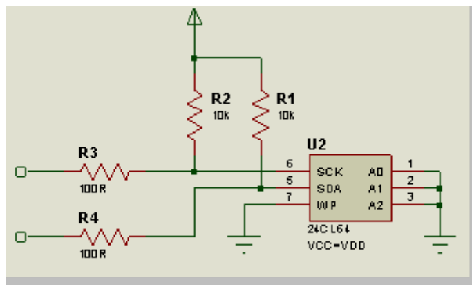
Schematic section with all parts / terminals placed
