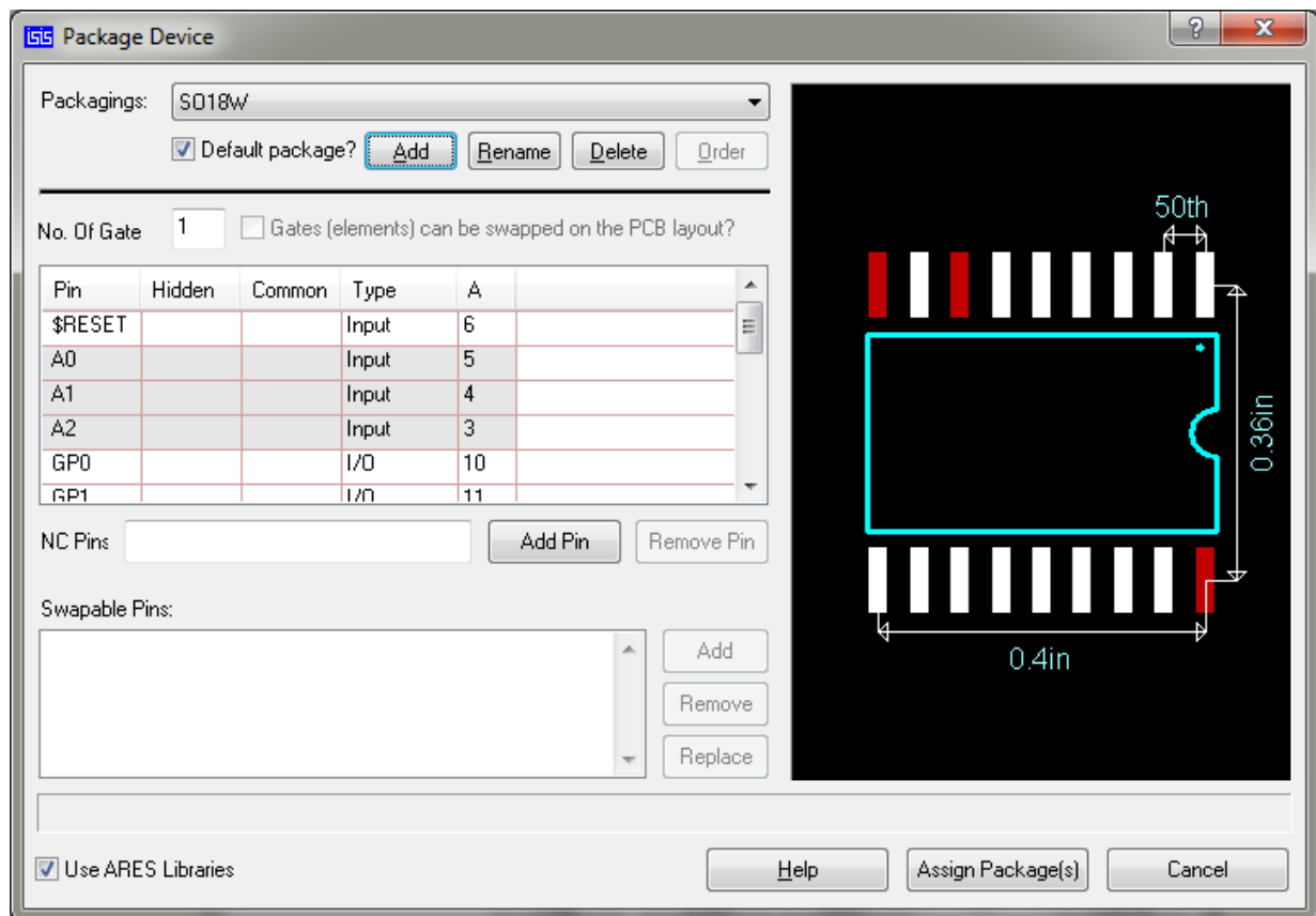
Selecting the SO18W from the package library
