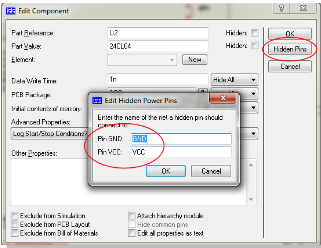
Hidden Power pins in schematic components.
