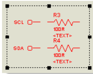
Dragging components
