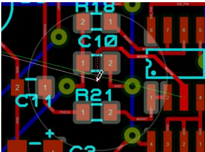
Push Mode (Imovable ojects only)
