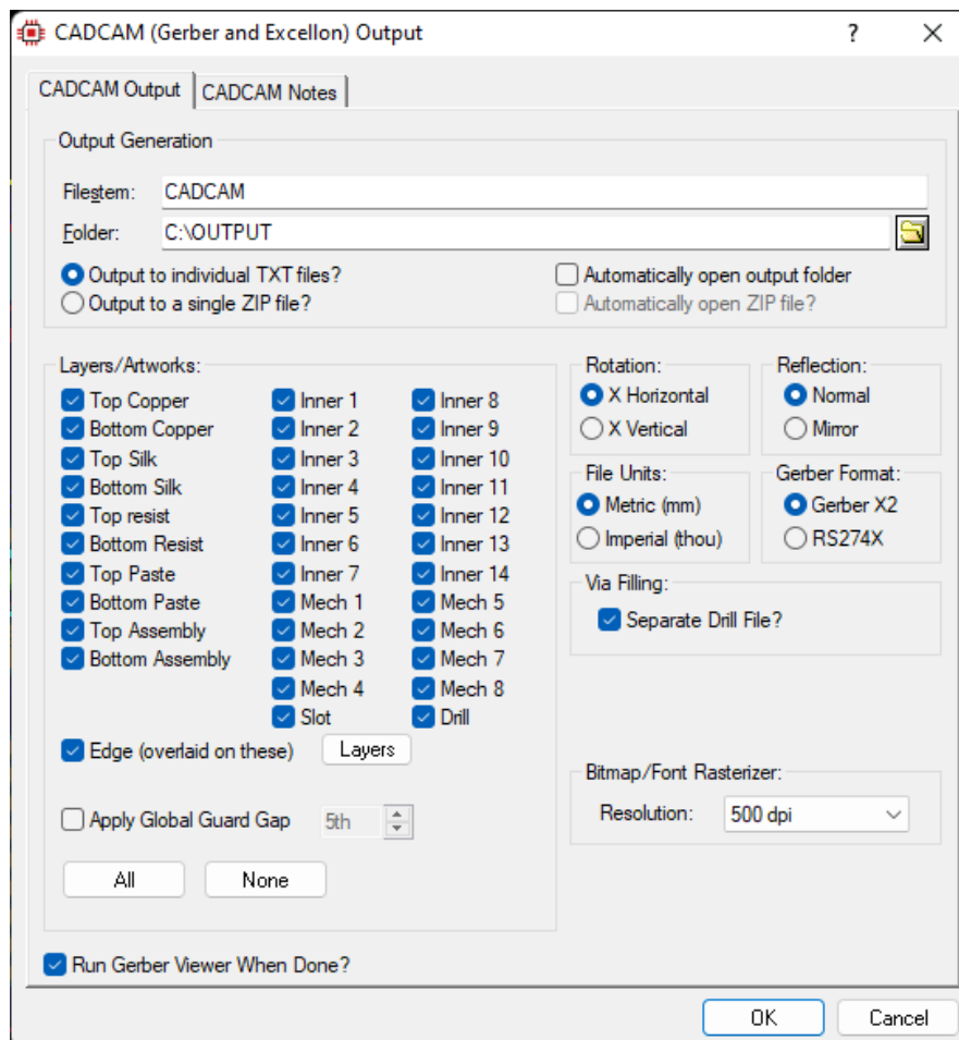
The Gerber / Excellon Output dialogue form
