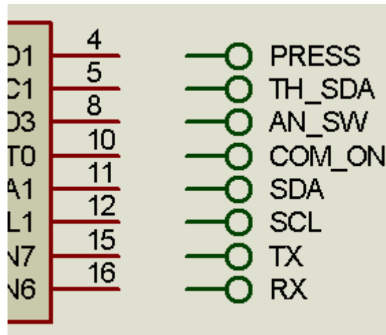
Terminals belonging to the dsPIC33
