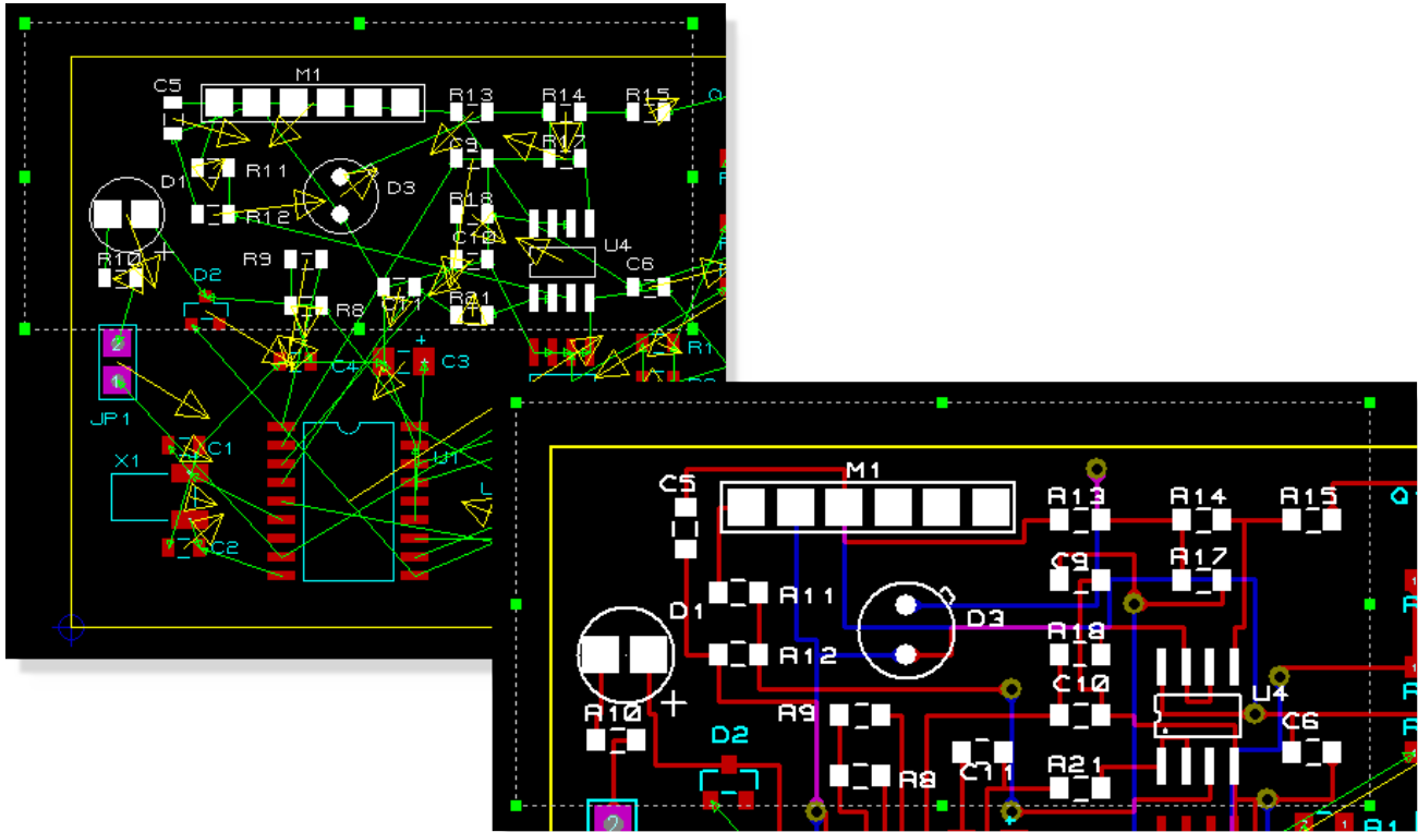
Autorouting an area of the board
