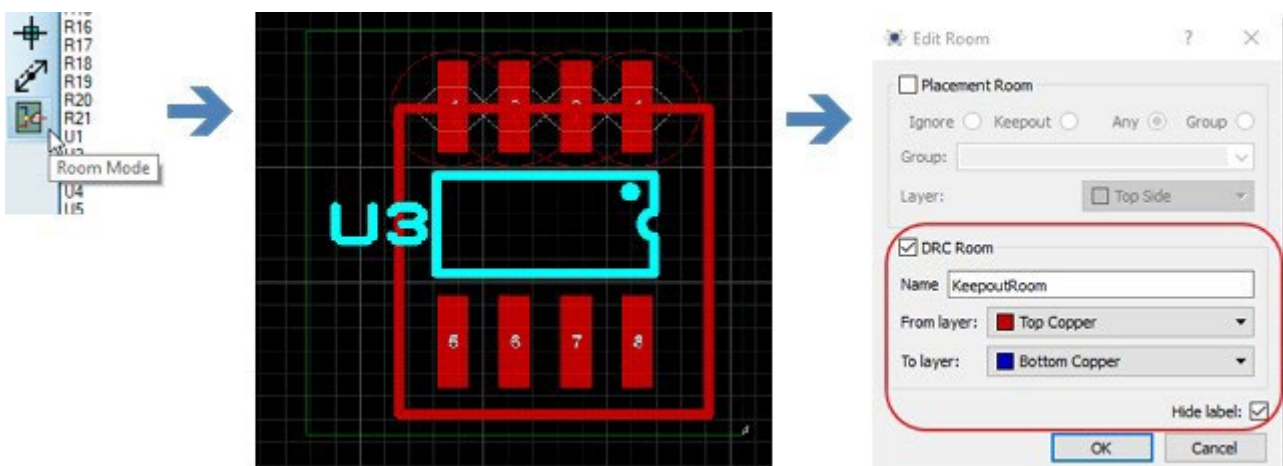
Setting up a Design Rule Room
